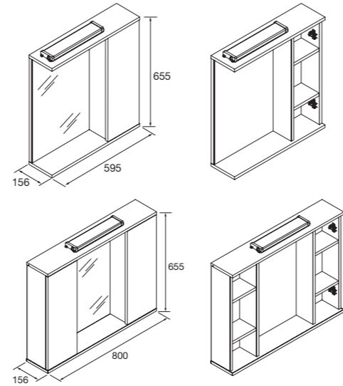
Cabinet Loira 600 1 door glossy white 2 halogen spotlights with switch IP44 - 6W 595x655x156 97367 172 €
