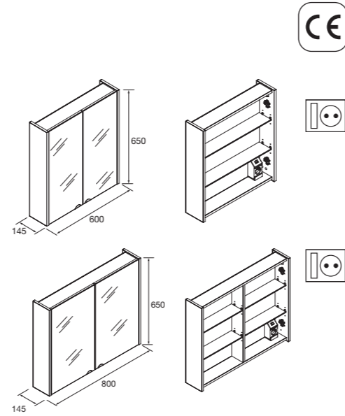
Cabinet SCHWAN 600 2 doors, mirror with switch and socket IP 44 600x650x145 24066 267 €
